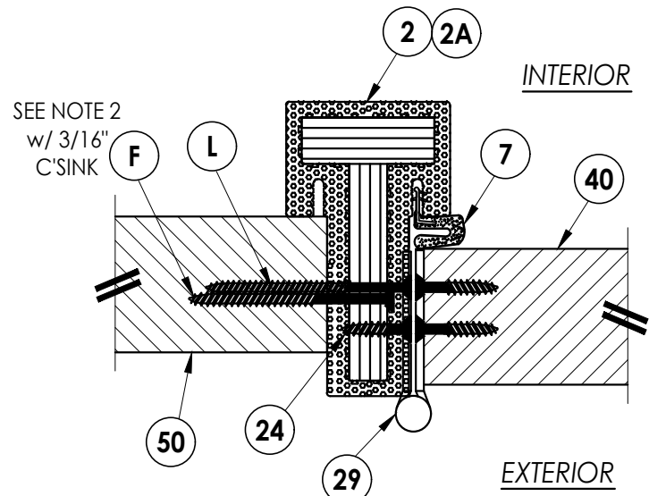
2 3 HORIZONTAL CROSS SECTION Type B (1 or 1.5") Integral Mullion Outswing
