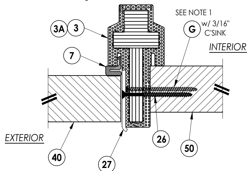
5 3 HORIZONTAL CROSS SECTION Type A (1 or 1.5") Integral Mullion Outswing
