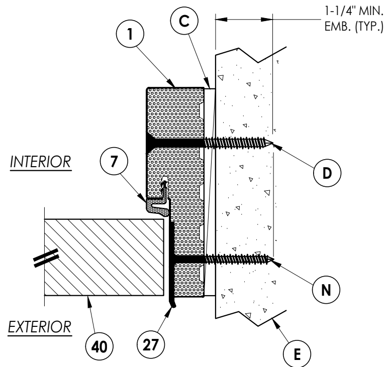
3 3 HORIZONTAL CROSS SECTION Shown Direct to masonry Outswing
