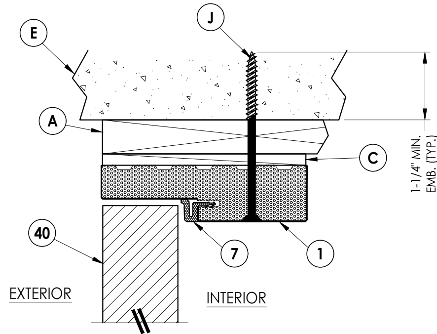
2 4 VERTICAL CROSS SECTION Shown with 1X Buck Outswing
