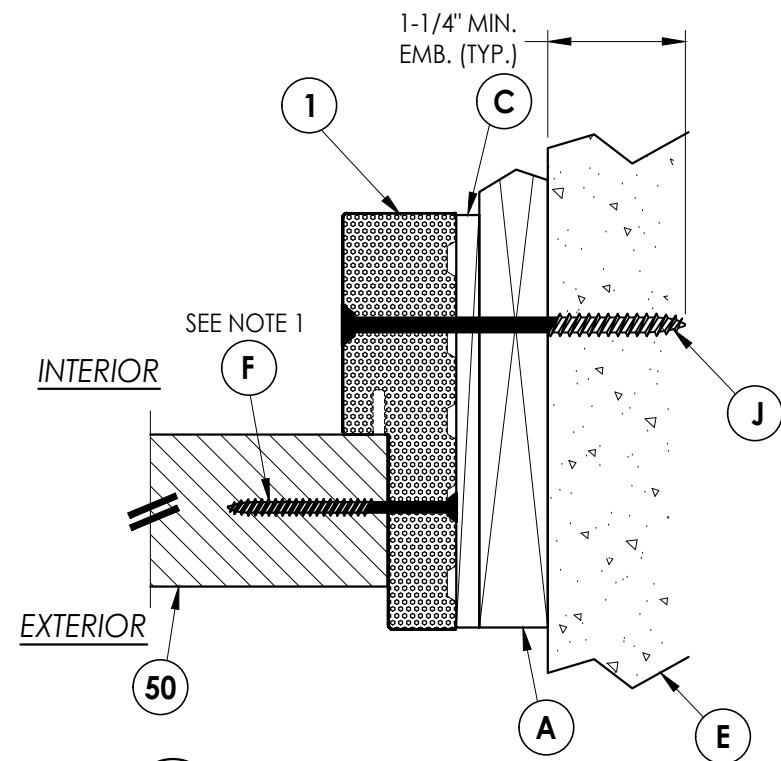
6 3 HORIZONTAL CROSS SECTION Shown with 1X Buck Outswing
